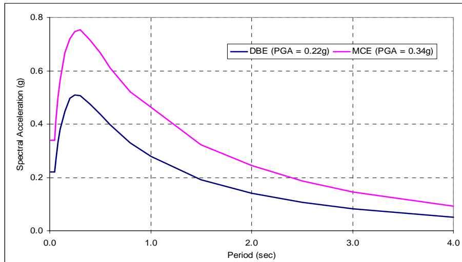
Figure 4: Response Spectra
