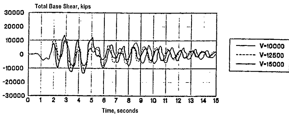
FIGURE 2A EFFECT OF SYSTEM STRENGTH ON BASE SHEAR RESPONSE
